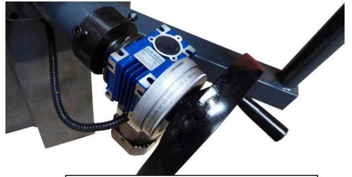
Detail of manual fine adjustment of downfeed with 0.0004" graduations. Wheelhead Elevation Motor shown.
