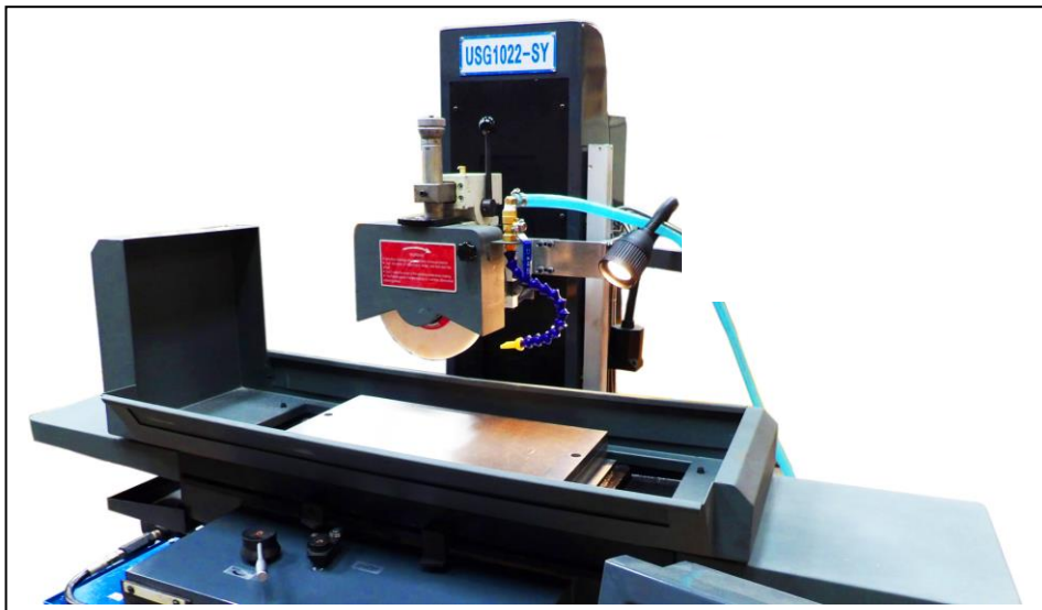
Detail showing permanent magnetic chuck, over wheel diamond dresser, flood coolant nozzle
